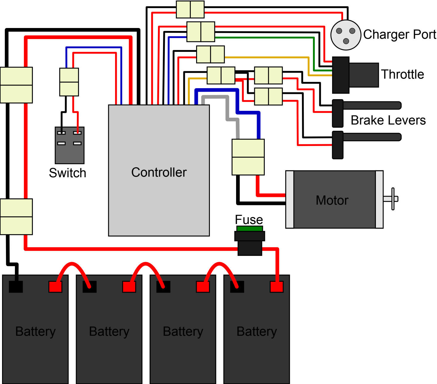
MX500-650-KIT5 Wiring Diagram
